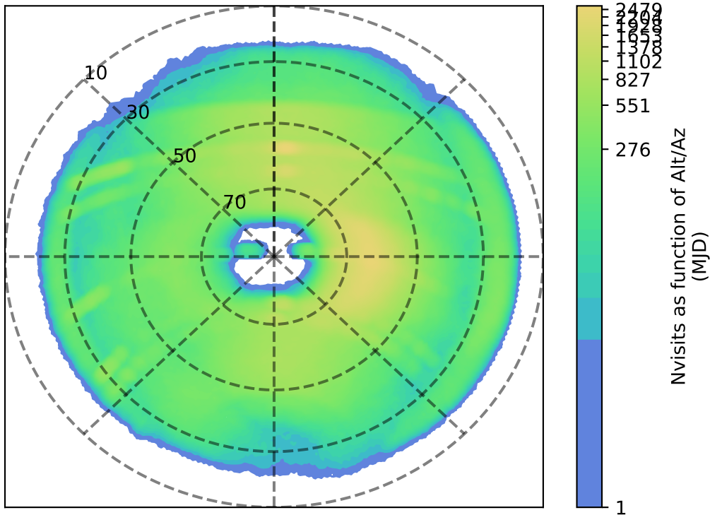
roll_pause_mjdp365_v3.4_10yrs i: Nvisits as function of Alt/Az
