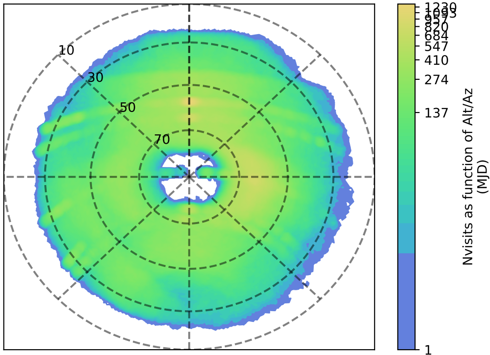
roll_pause_mjdp365_v3.4_10yrs g: Nvisits as function of Alt/Az
