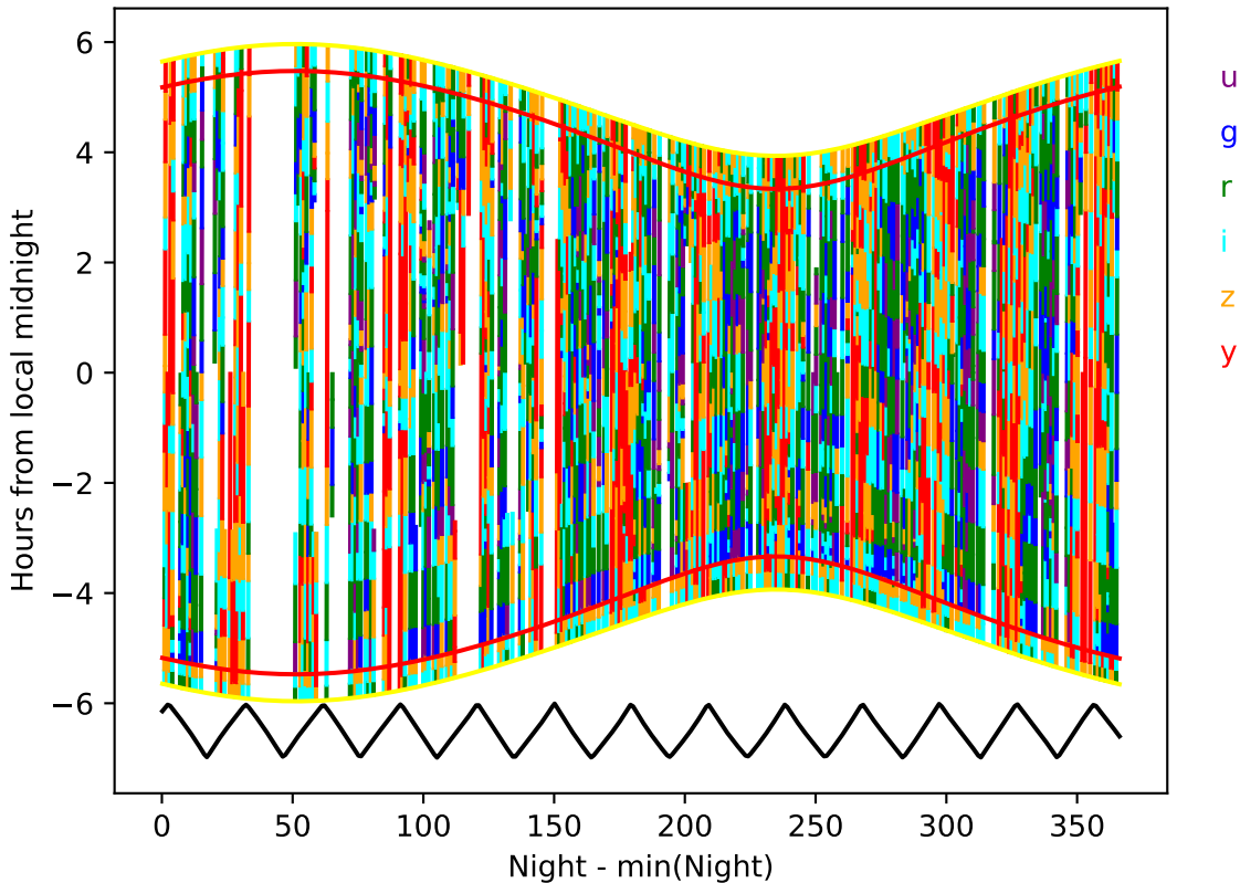
roll_pause_mjdp365_v3.4_10yrs year 8-9: Hourglass
