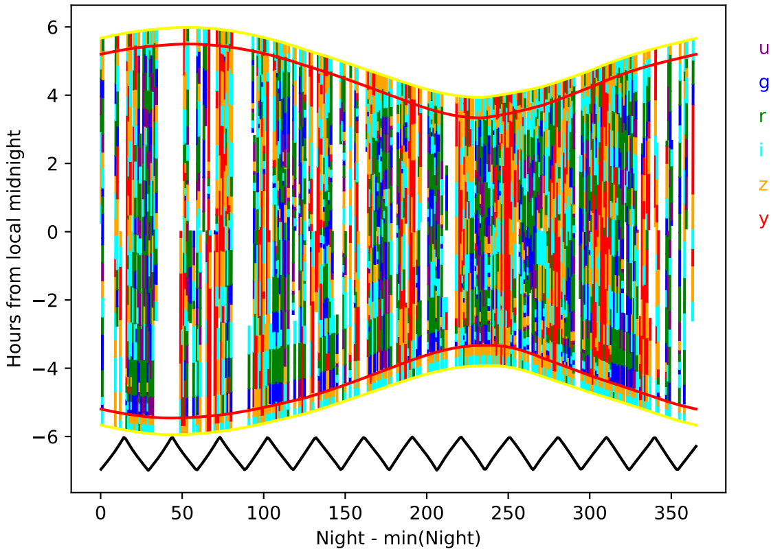
roll_pause_mjdp365_v3.4_10yrs year 4-5: Hourglass
