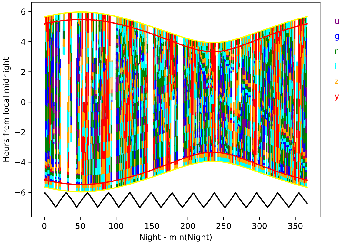
roll_pause_mjdp365_v3.4_10yrs year 0-1: Hourglass
