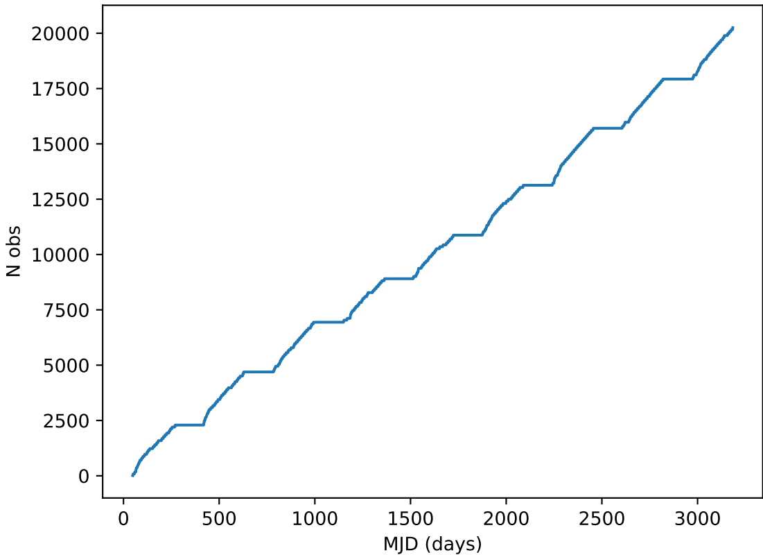
roll_pause_mjdp365_v3.4_10yrs note like DD:ELAISS1%: Cumulative
