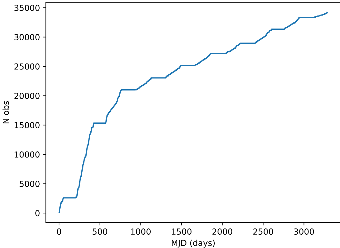
roll_pause_mjdp365_v3.4_10yrs note like DD: COSMOS%: Cumulative
