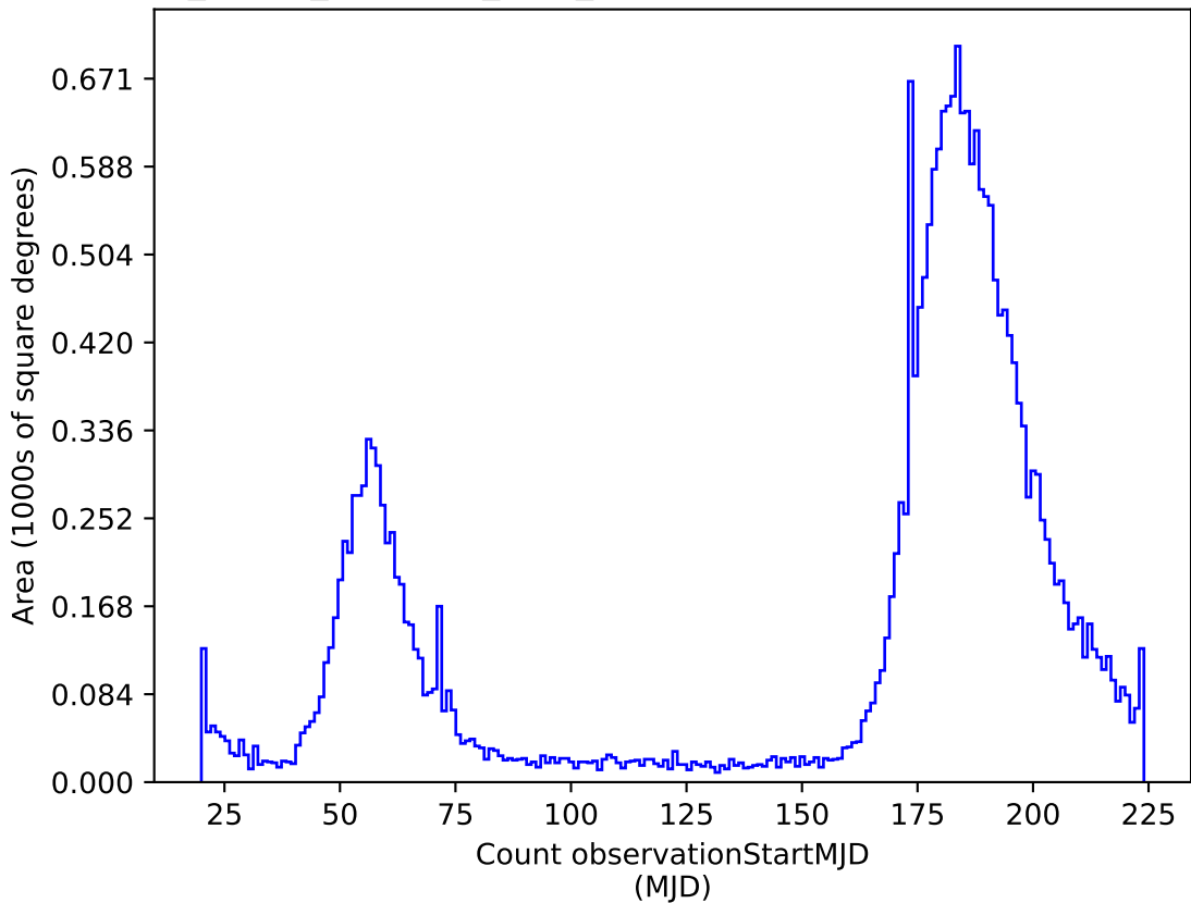
roll_pause_mjdp365_v3.4_10yrs r: Count observationStartMJD
