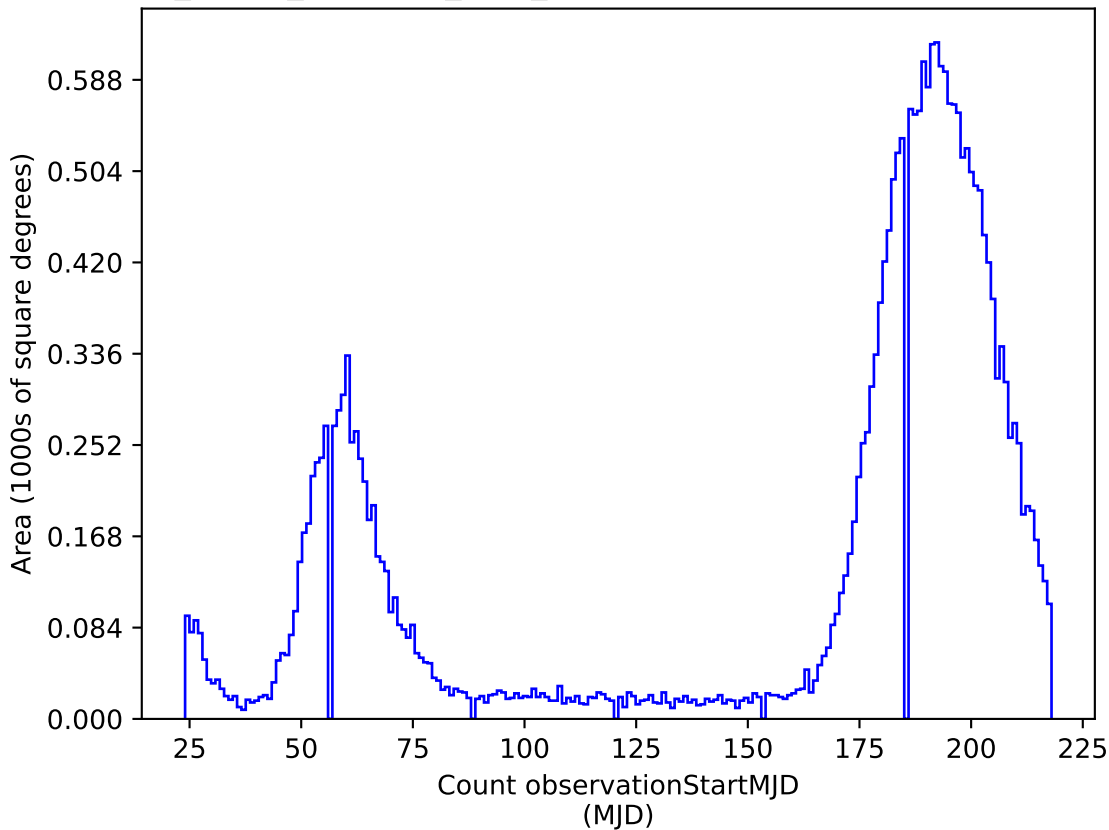
roll_pause_mjdp365_v3.4_10yrs i: Count observationStartMJD
