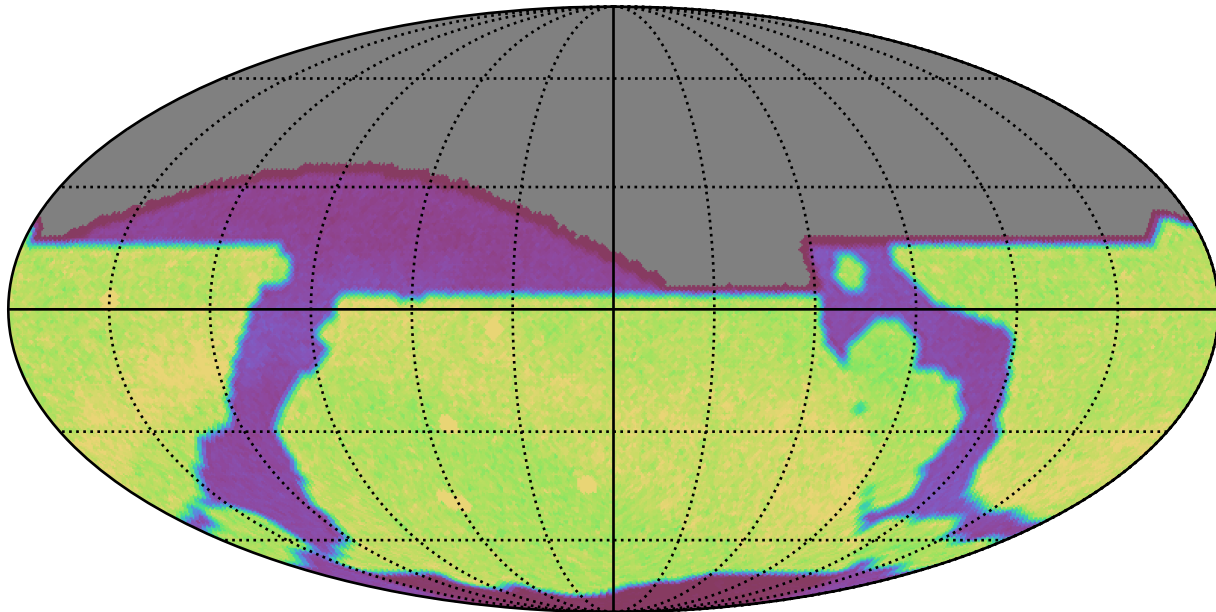
roll_pause_mjdp365_v3.4_10yrs : Count observationStartMJD
