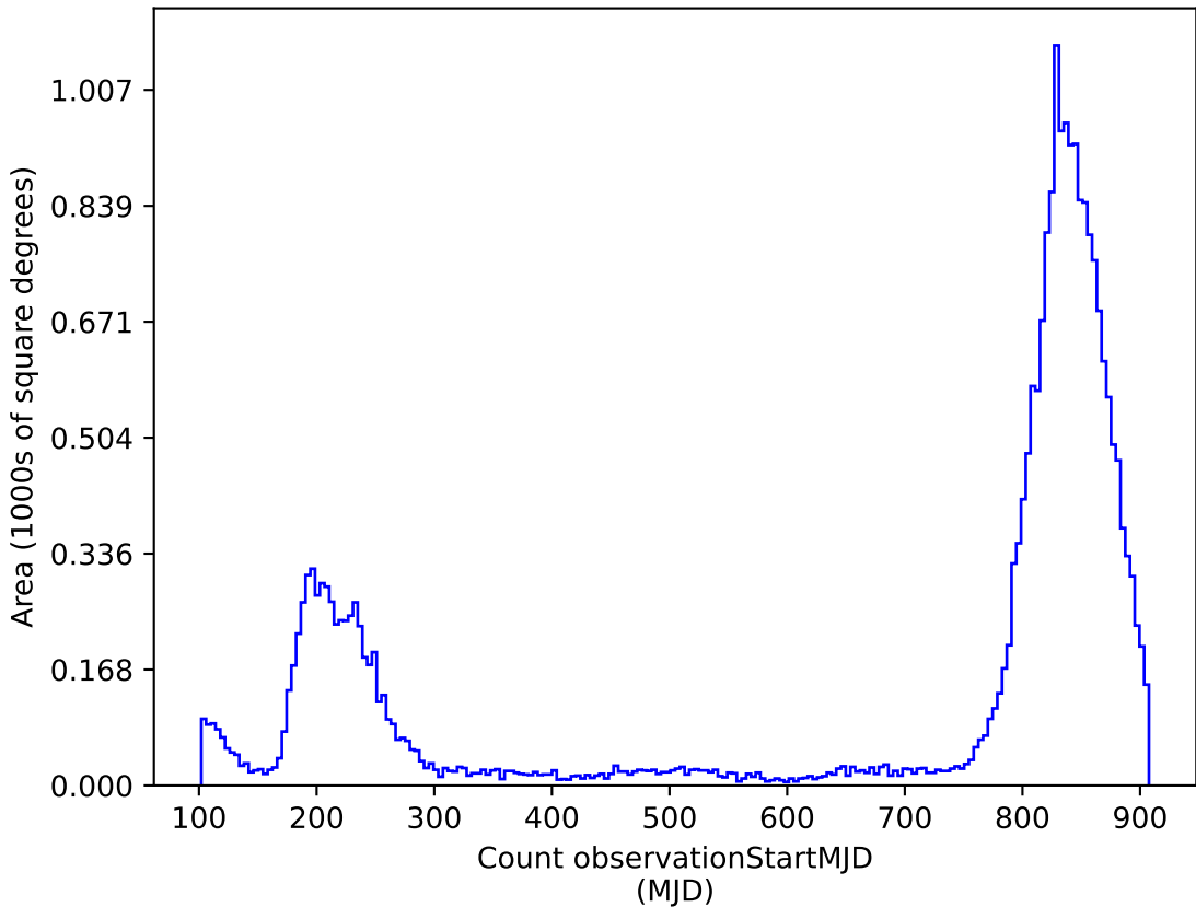
roll_pause_mjdp365_v3.4_10yrs : Count observationStartMJD
