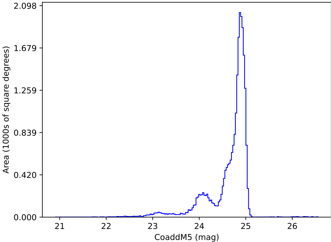
roll_pause_mjdp365_v3.4_10yrs y: CoaddM5
