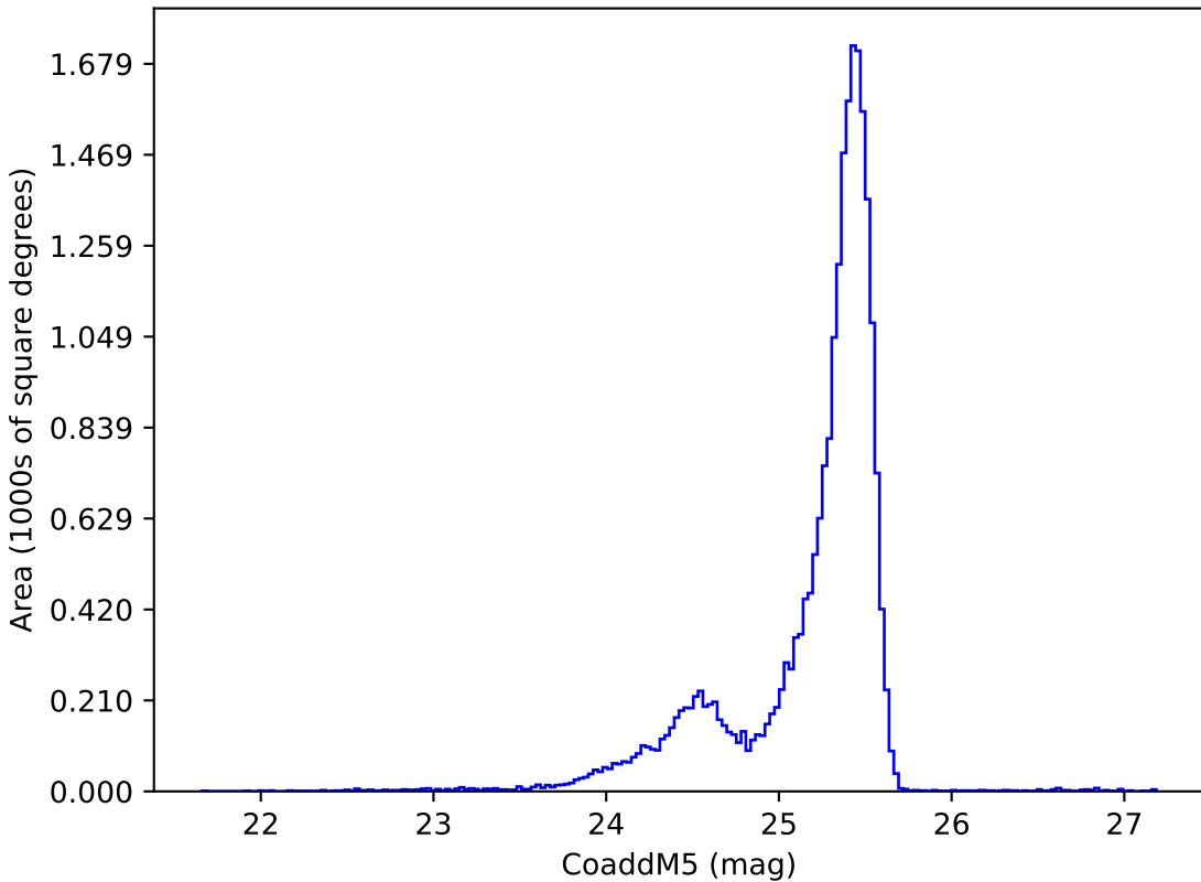
roll_pause_mjdp365_v3.4_10yrs u: CoaddM5
