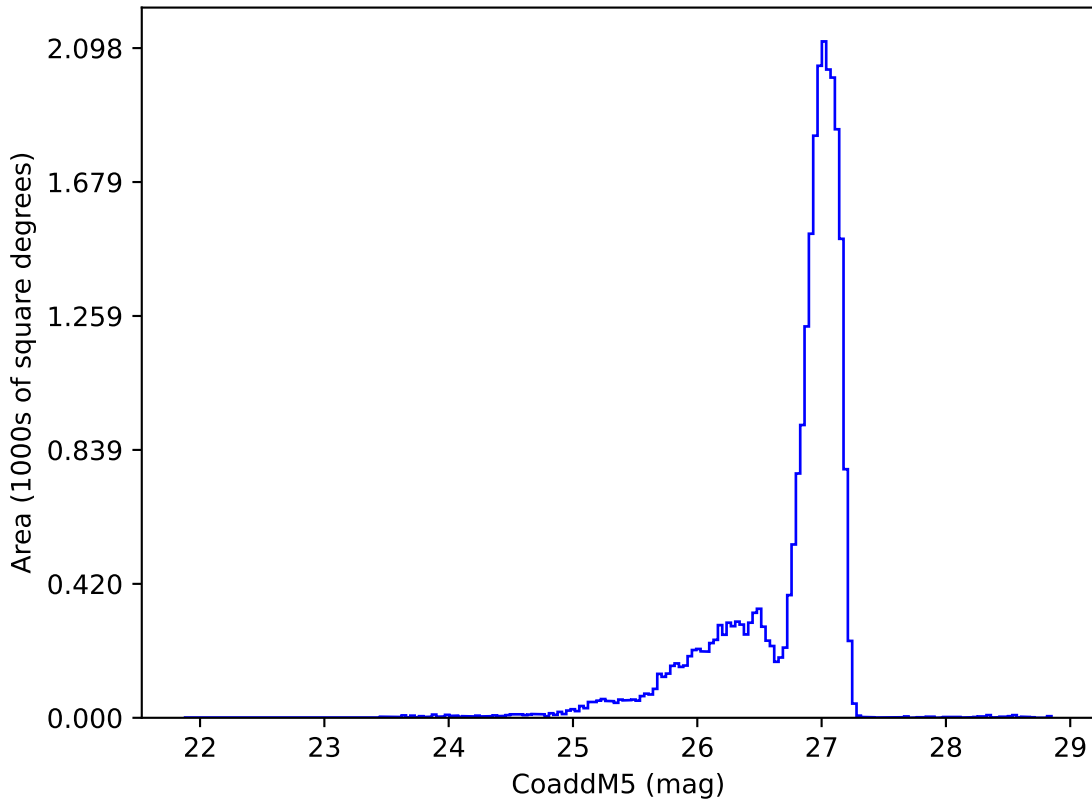
roll_pause_mjdp365_v3.4_10yrs r: CoaddM5
