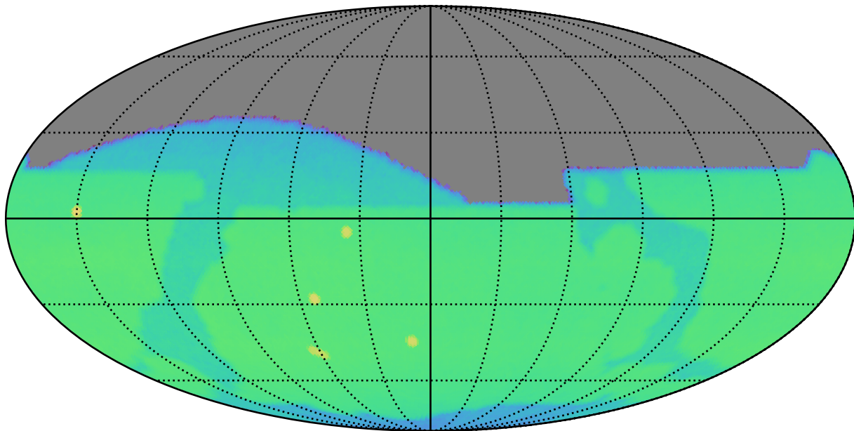
roll_pause_mjdp365_v3.4_10yrs i: CoaddM5
