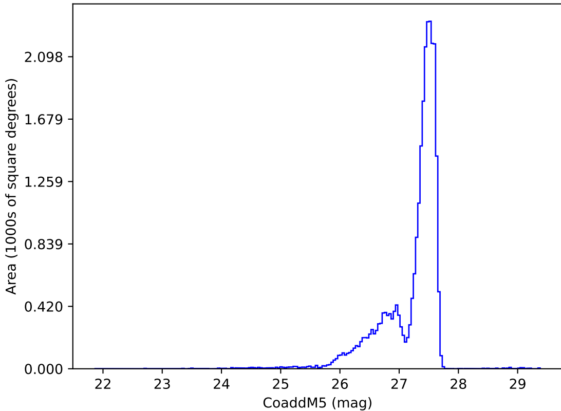
roll_pause_mjdp365_v3.4_10yrs : CoaddM5
