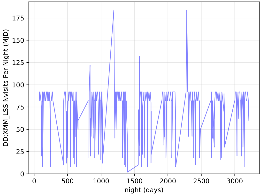
roll_pause_mjdp365_v3.4_10yrs all bands: DD:XMM_LSS Nvisits Per Night
