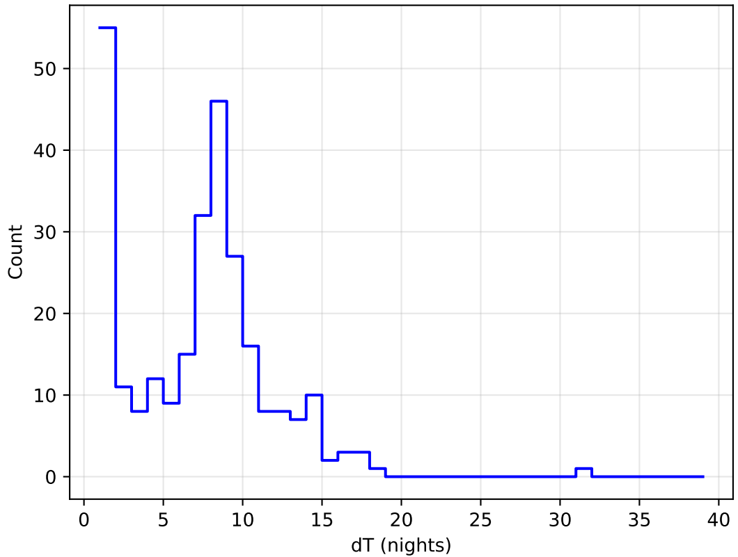
roll_pause_mjdp365_v3.4_10yrs all bands: DD:XMM_LSS Delta Nights Histogram
