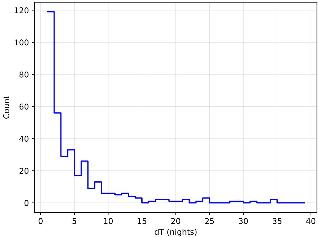
roll_pause_mjdp365_v3.4_10yrs all bands: DD:WFD Delta Nights Histogram
