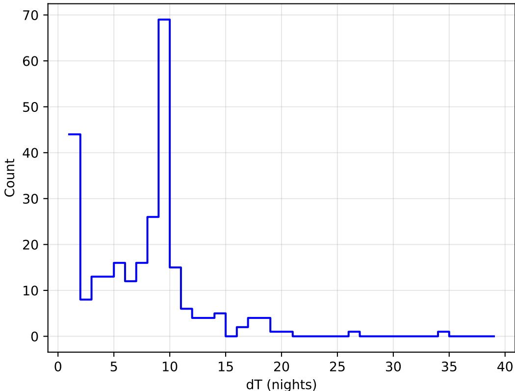
roll_pause_mjdp365_v3.4_10yrs all bands: DD:ELAISS1 Delta Nights Histogram
