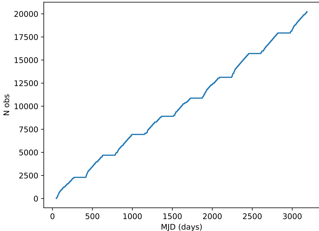
roll_pause_mjdp365_v3.4_10yrs all bands: DD:ELAISS1 Cumulative NVisits
