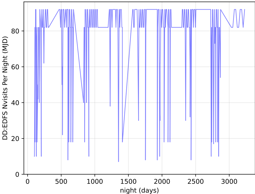
roll_pause_mjdp365_v3.4_10yrs all bands: DD:EDFS Nvisits Per Night
