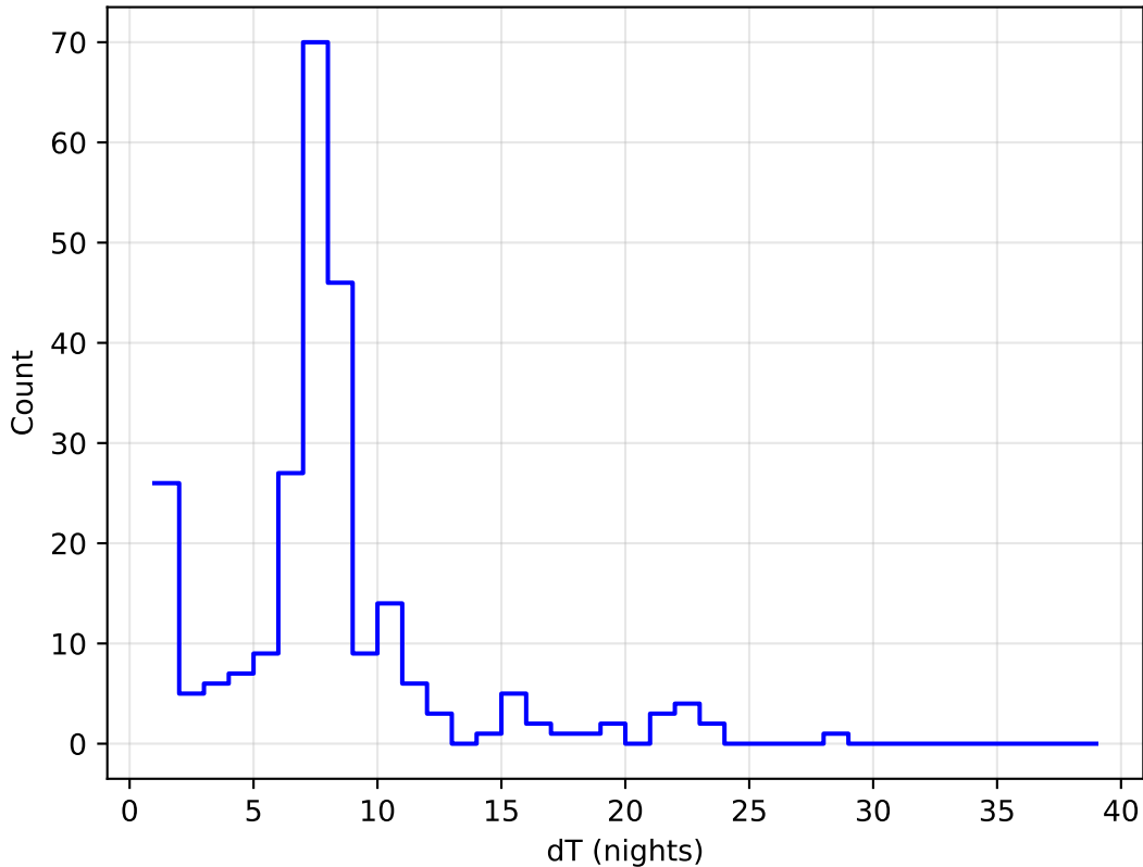
roll_pause_mjdp365_v3.4_10yrs all bands: DD:EDFS Delta Nights Histogram
