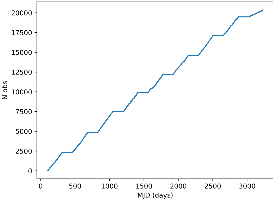
roll_pause_mjdp365_v3.4_10yrs all bands: DD:EDFS Cumulative NVisits
