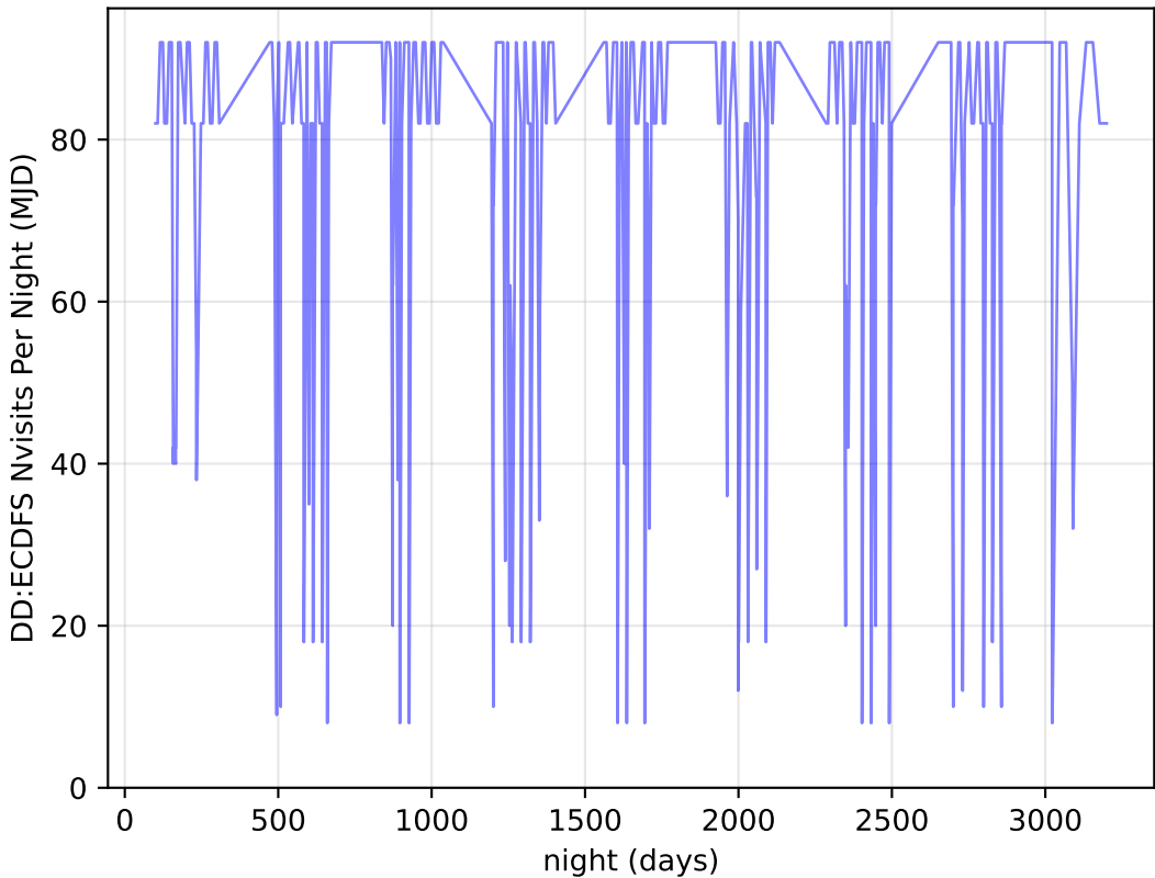
roll_pause_mjdp365_v3.4_10yrs all bands: DD:ECDFS Nvisits Per Night
