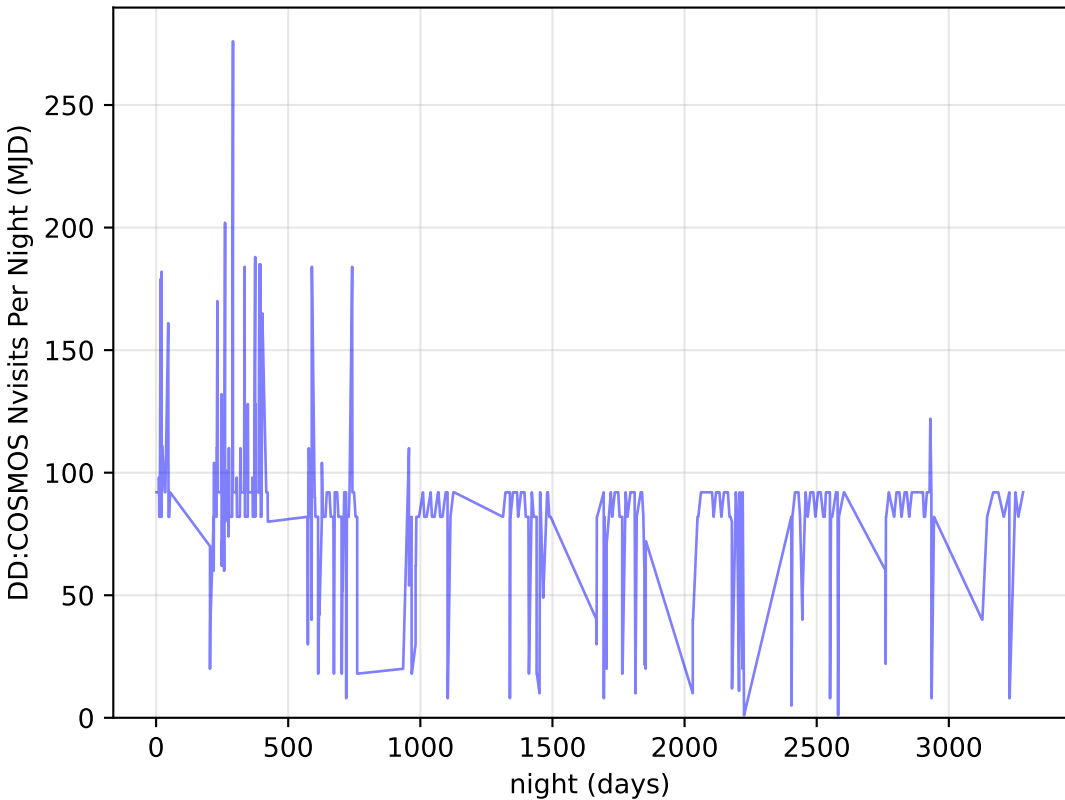
roll_pause_mjdp365_v3.4_10yrs all bands: DD: COSMOS Nvisits Per Night
