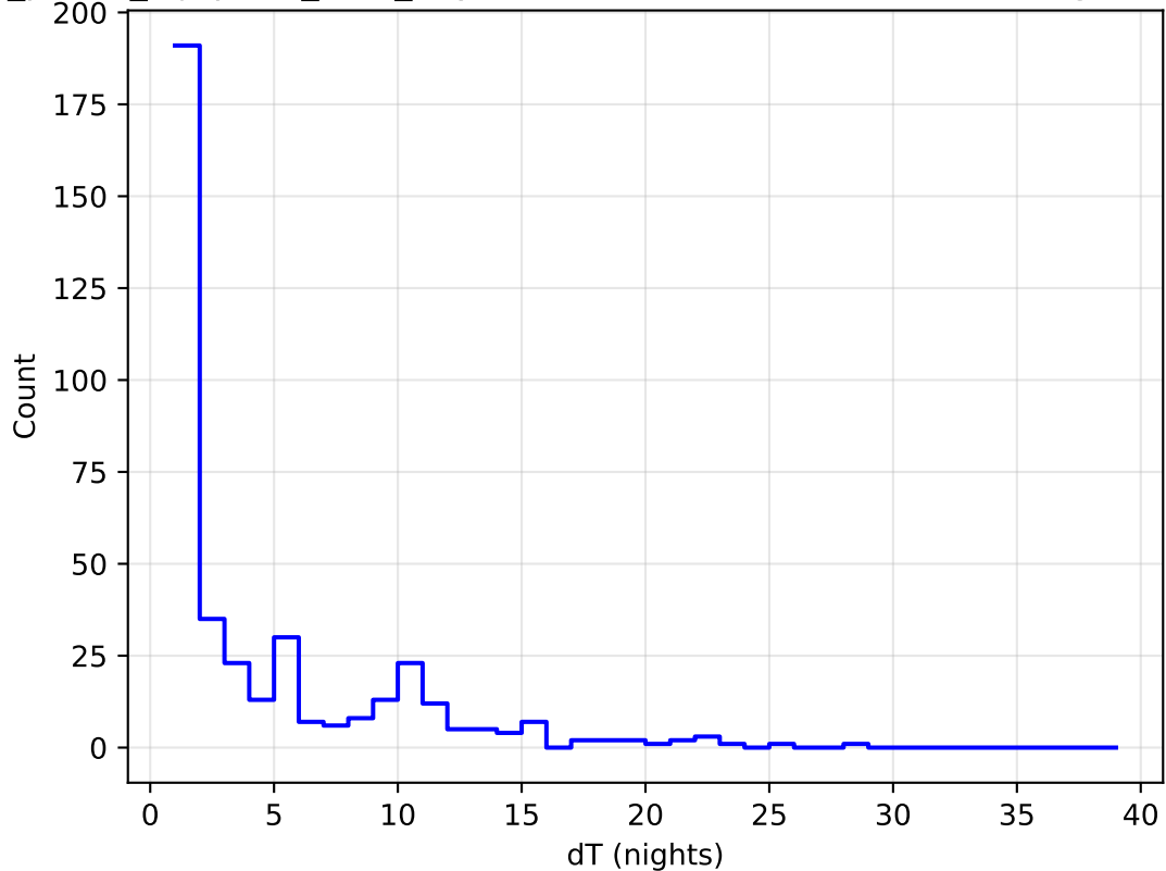
roll_pause_mjdp365_v3.4_10yrs all bands: DD:COSMOS Delta Nights Histogram
