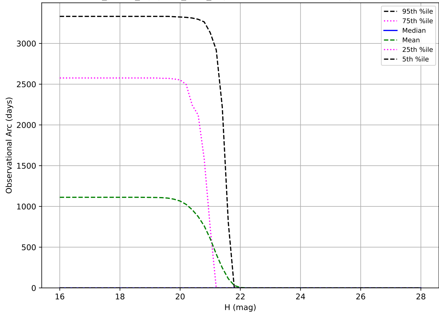
roll_pause_mjdp270_v3.4_10yrs: Observational Arc Length Vatira
