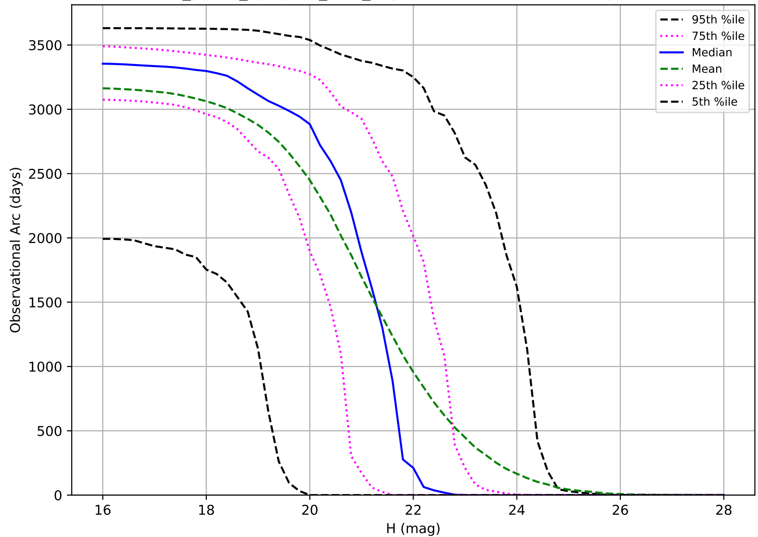
roll_pause_mjdp270_v3.4_10yrs: Observational Arc Length PHA
