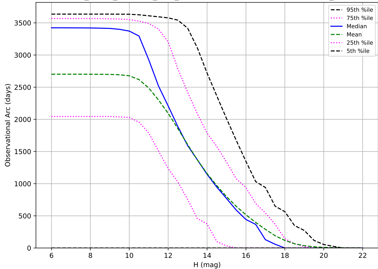
roll_pause_mjdp270_v3.4_10yrs: Observational Arc Length OCC_r5
