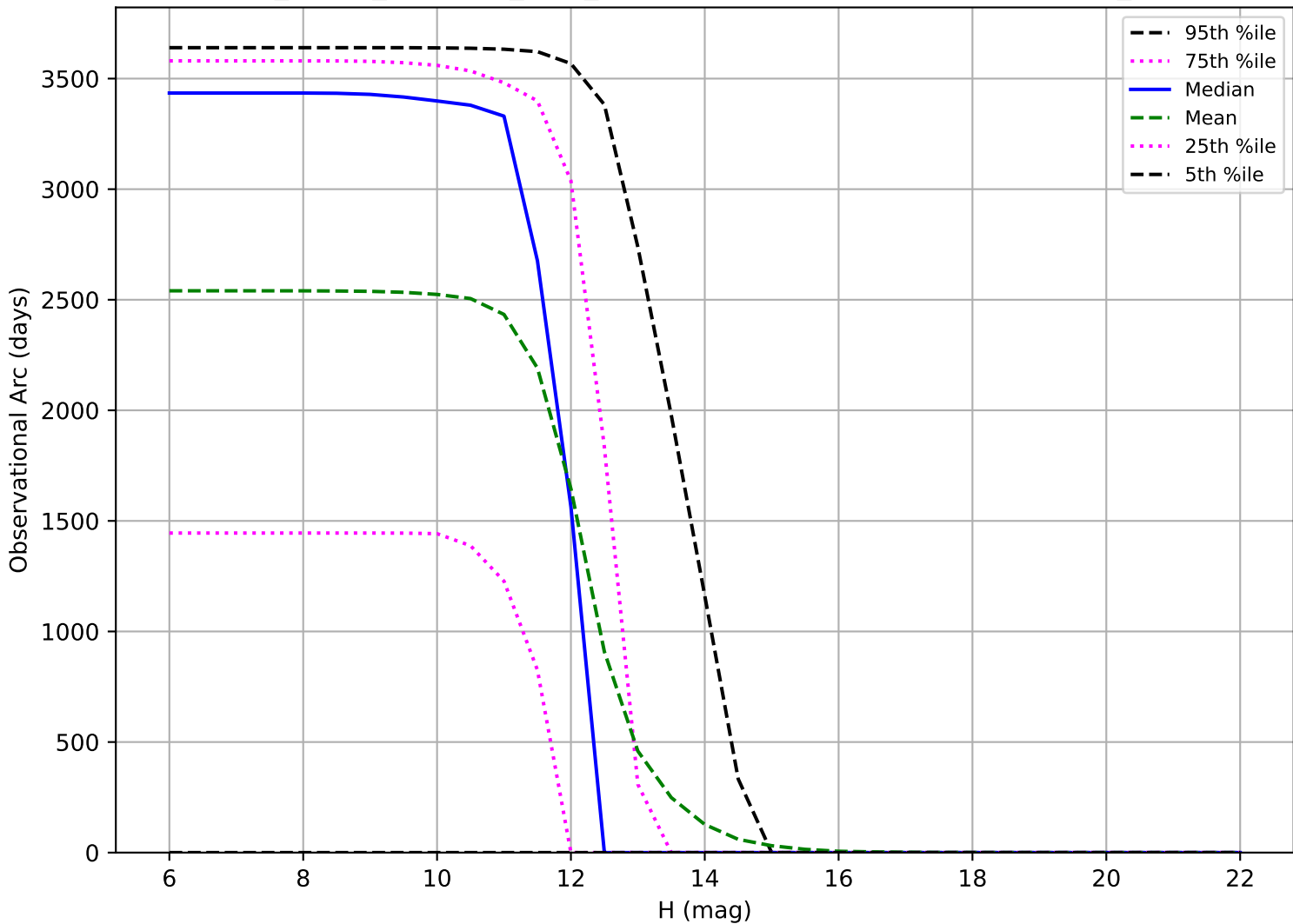
roll_pause_mjdp270_v3.4_10yrs: Observational Arc Length OCC_r20
