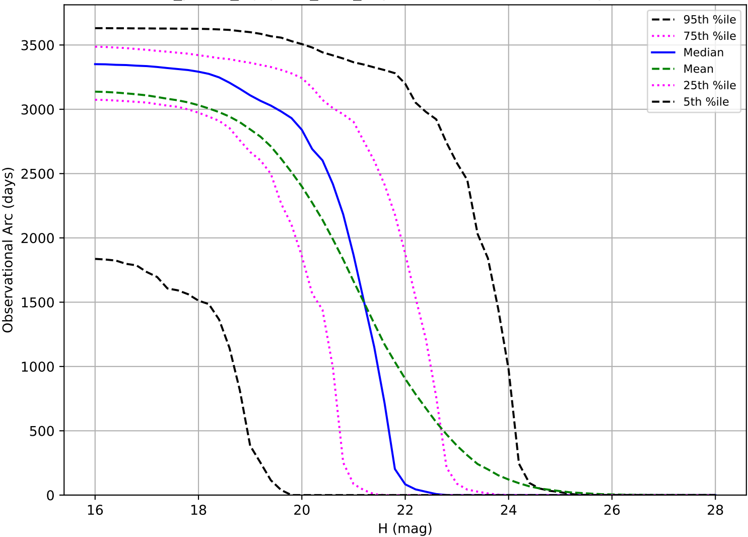
roll_pause_mjdp270_v3.4_10yrs: Observational Arc Length NEO
