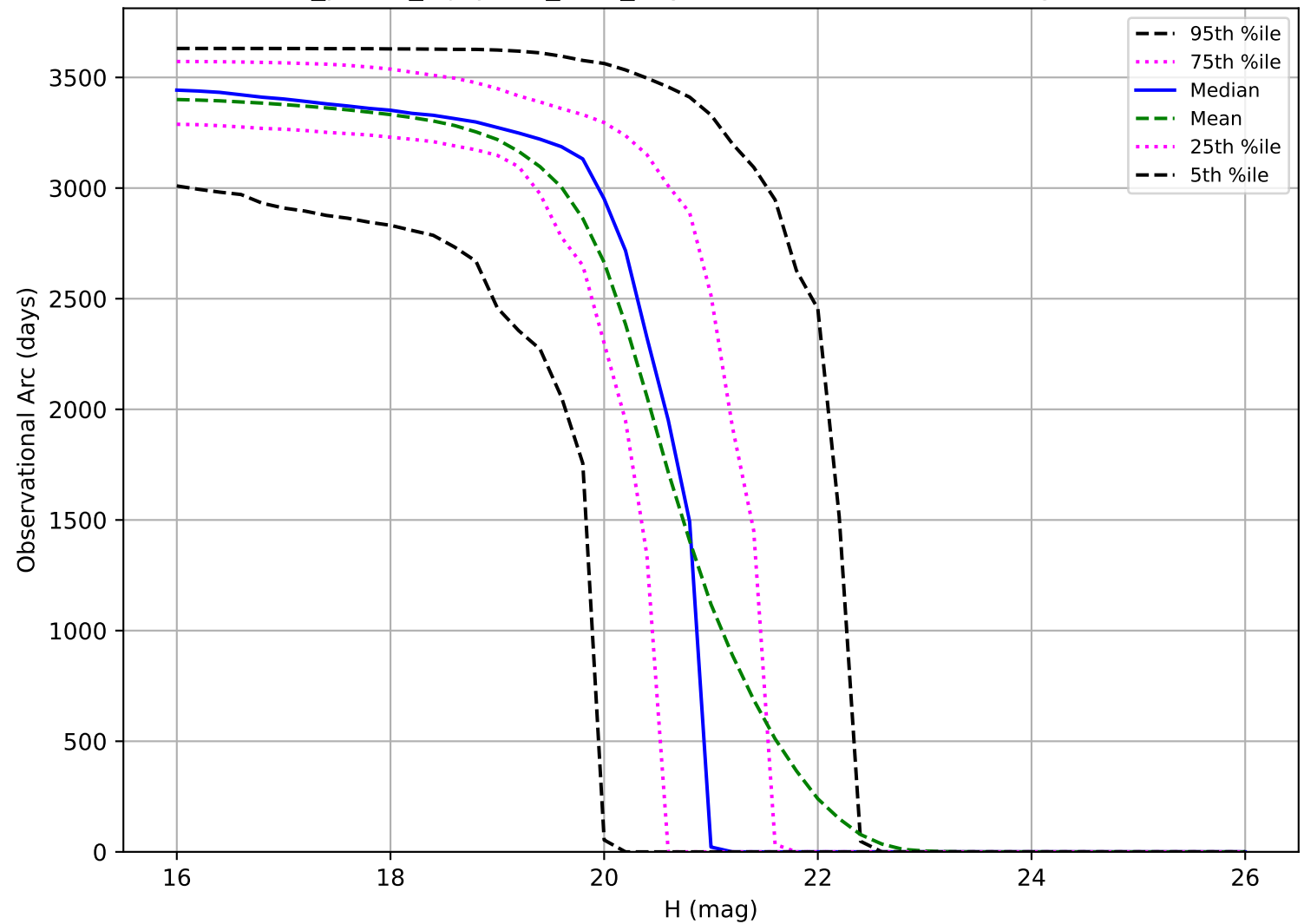
roll_pause_mjdp270_v3.4_10yrs: Observational Arc Length MBA
