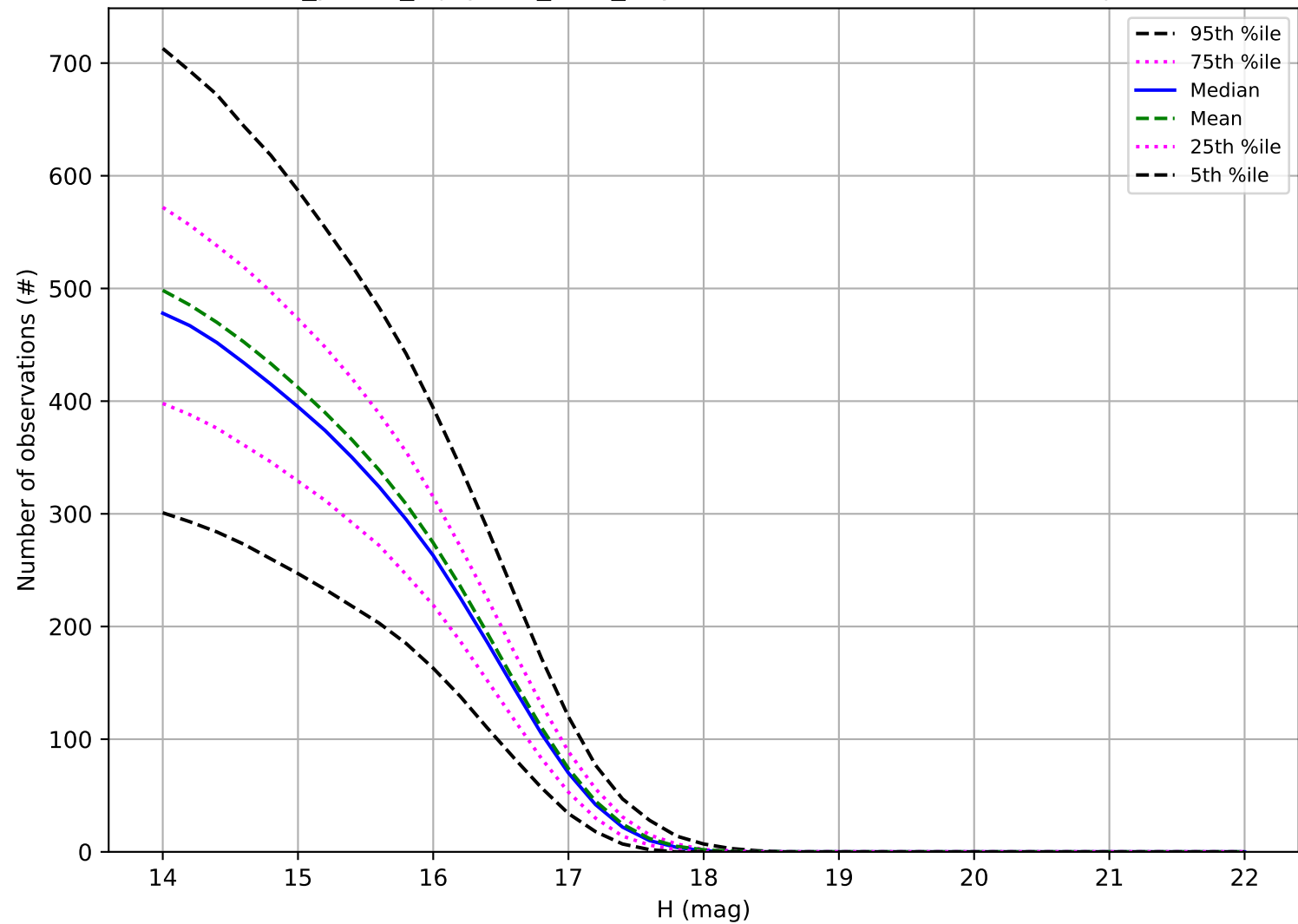
roll_pause_mjdp270_v3.4_10yrs: Number of observations Trojan
