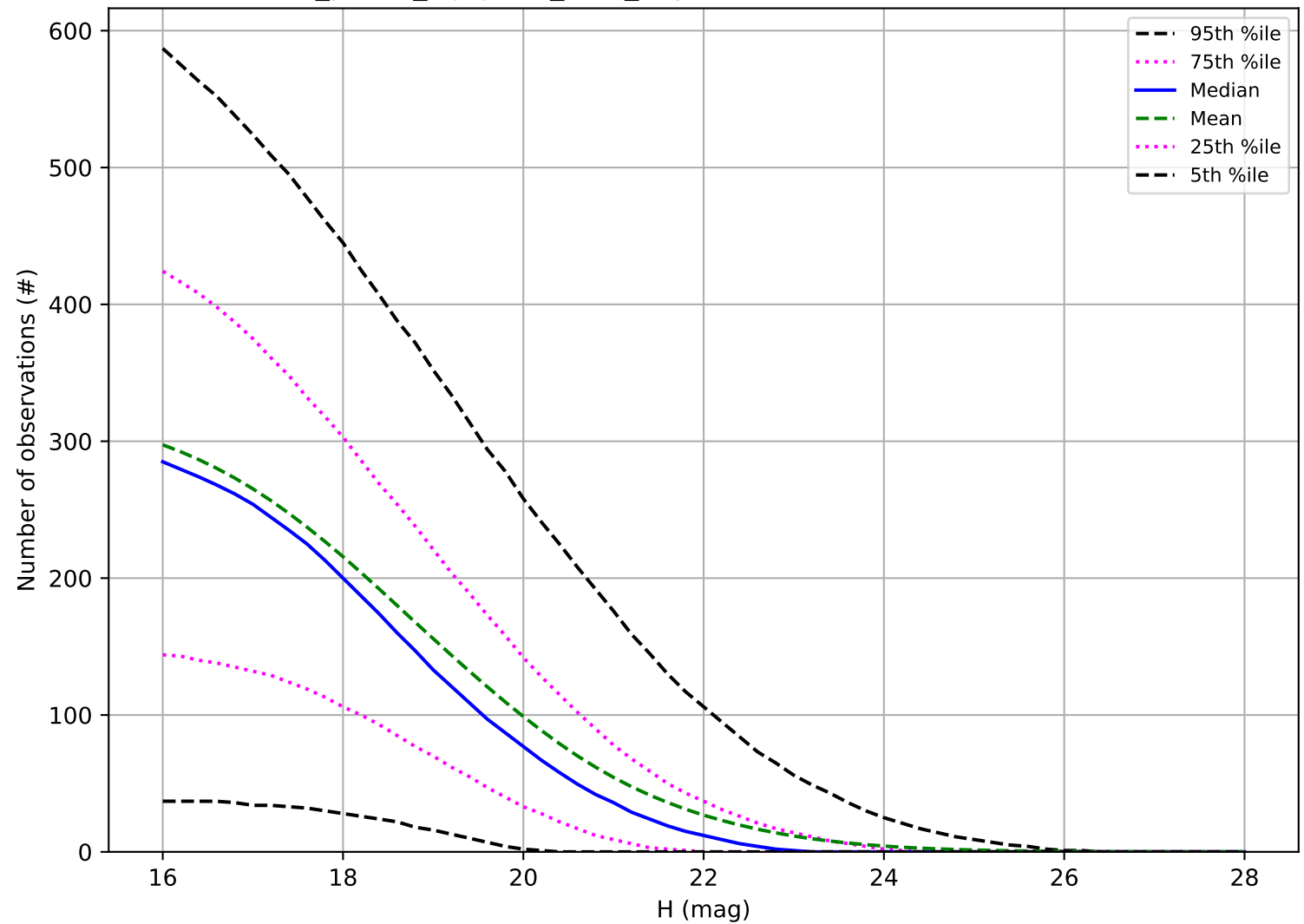
roll_pause_mjdp270_v3.4_10yrs: Number of observations PHA
