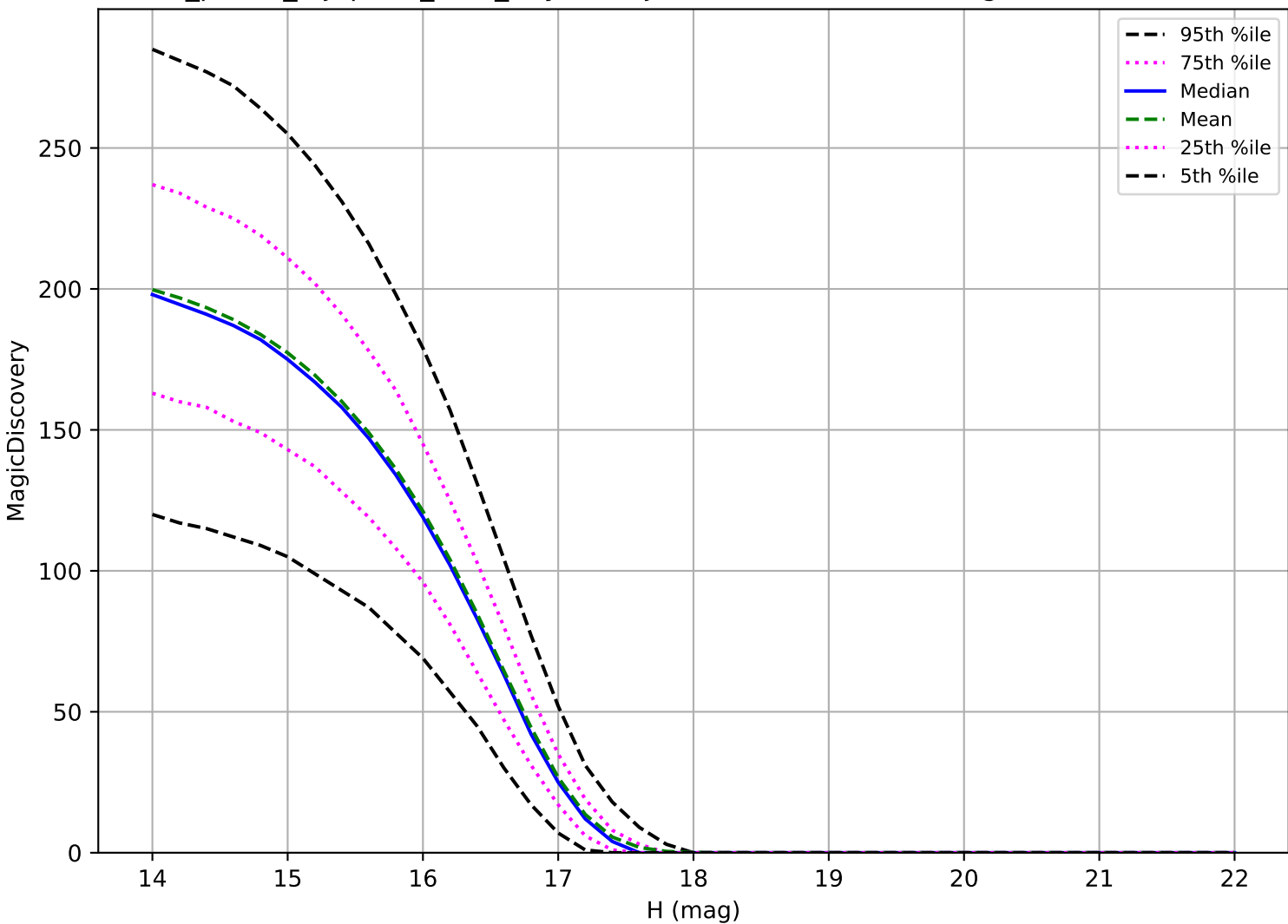
roll_pause_mjdp270_v3.4_10yrs: Trojan 6 detections in 60 nights detection loss
