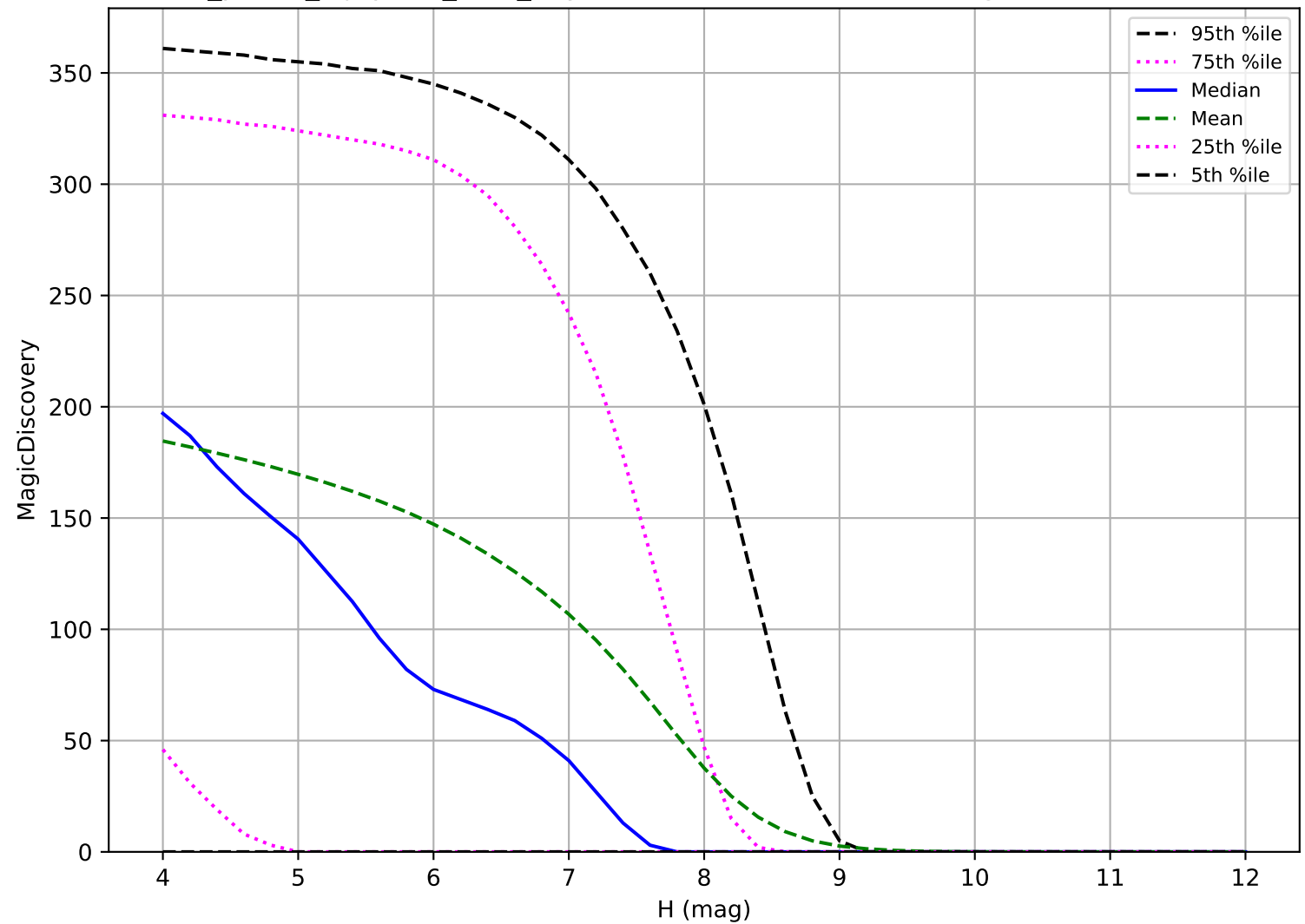
roll_pause_mjdp270_v3.4_10yrs: TNO 6 detections in 60 nights detection loss
