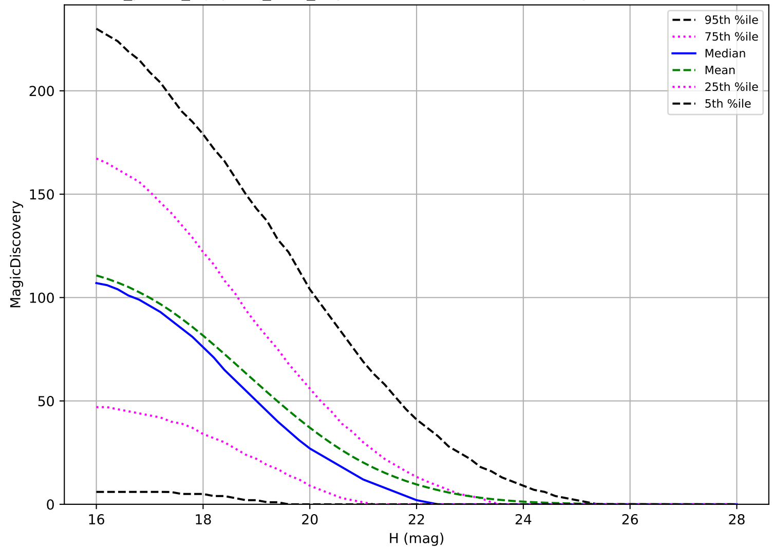
roll_pause_mjdp270_v3.4_10yrs: PHA 6 detections in 60 nights detection loss
