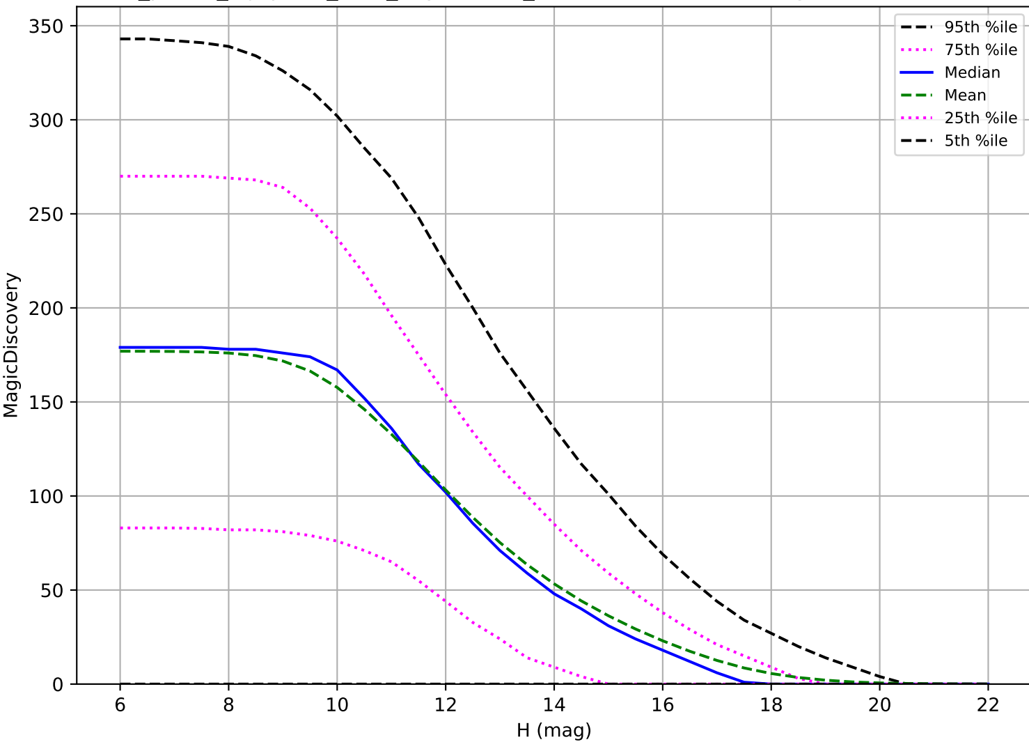
roll_pause_mjdp270_v3.4_10yrs: OCC_r5 6 detections in 60 nights detection loss
