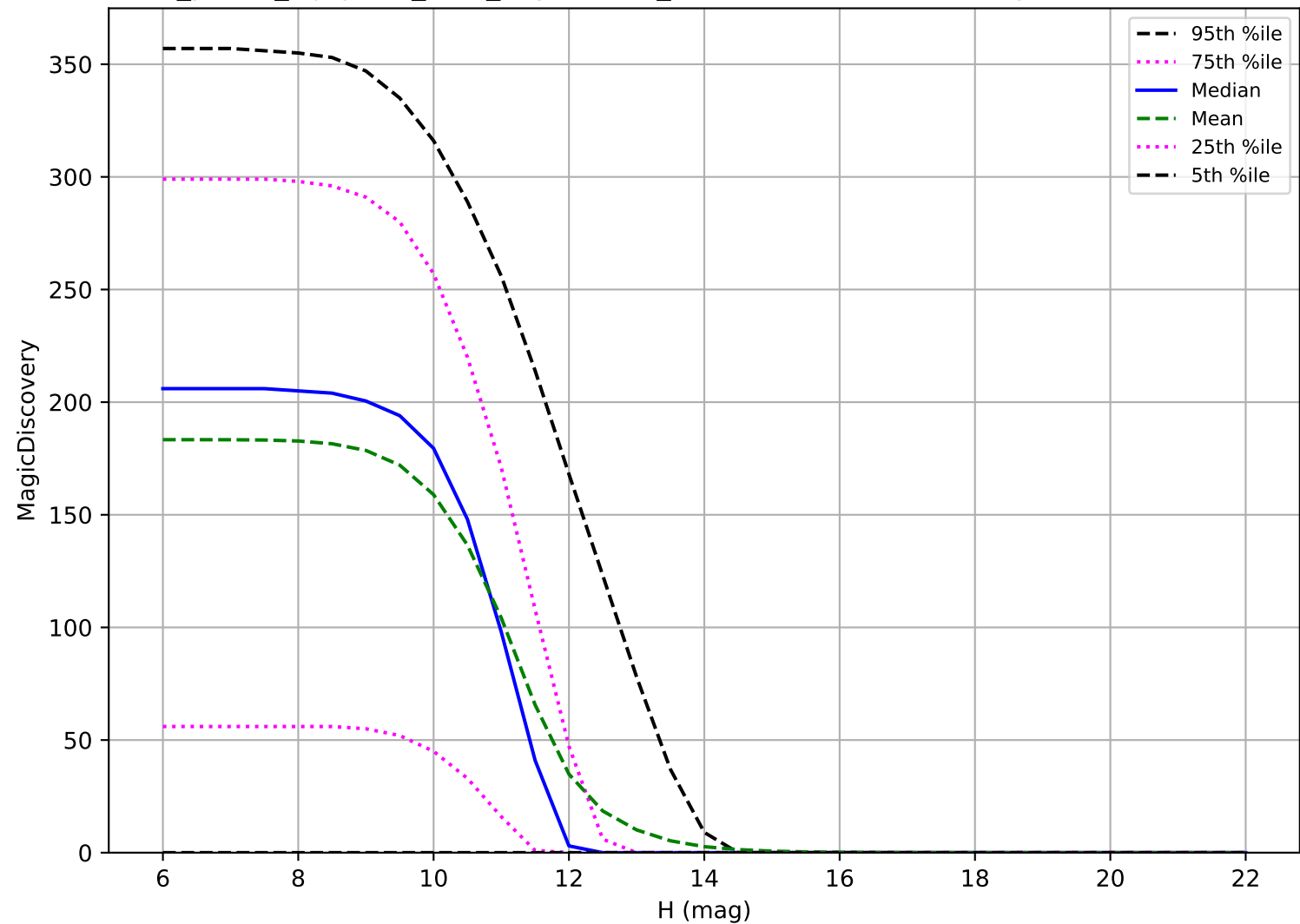
roll_pause_mjdp270_v3.4_10yrs: OCC_r20 6 detections in 60 nights detection loss
