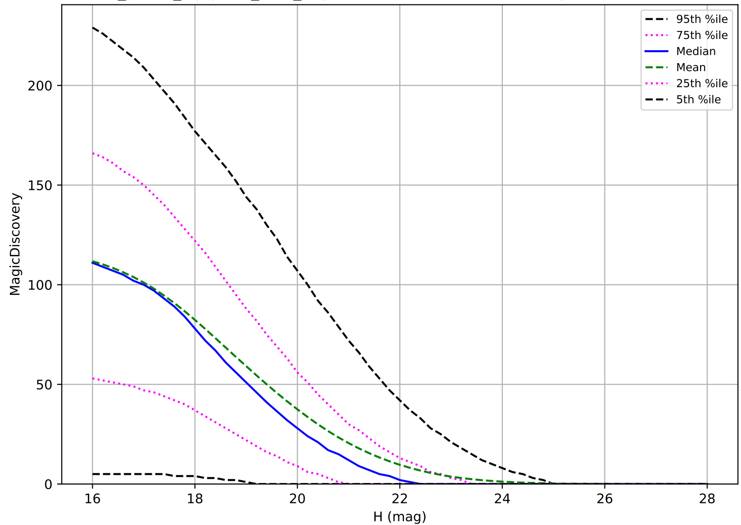
roll_pause_mjdp270_v3.4_10yrs: NEO 6 detections in 60 nights detection loss
