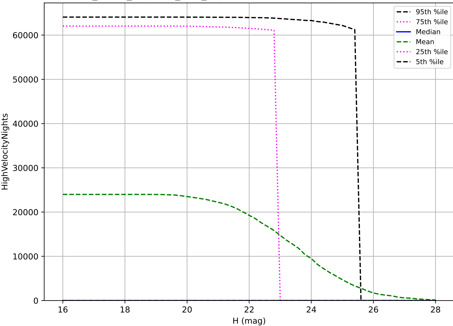
roll_pause_mjdp270_v3.4_10yrs: PHA High velocity pair detection loss
