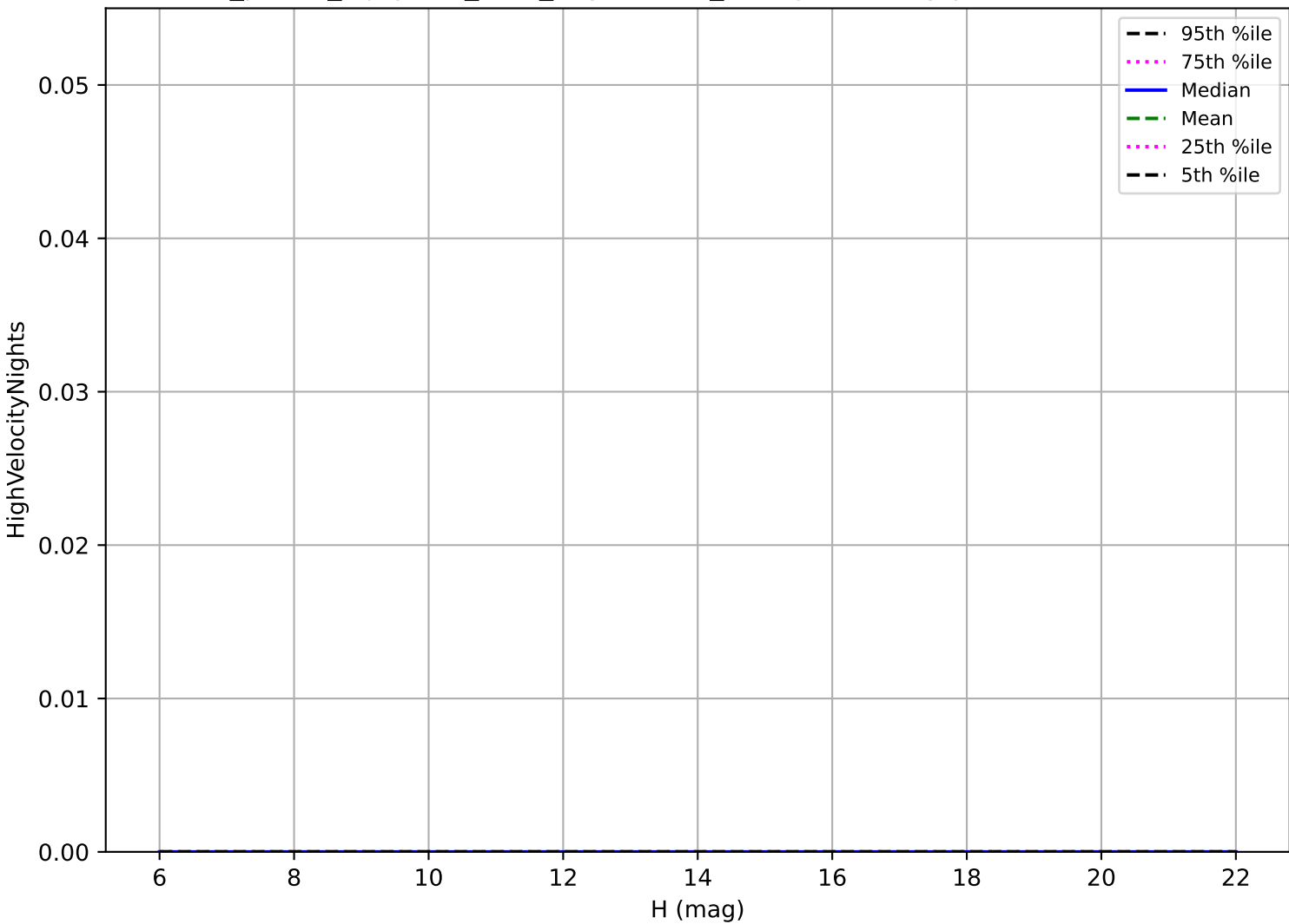
roll_pause_mjdp270_v3.4_10yrs: OCC_r5 High velocity pair detection loss
