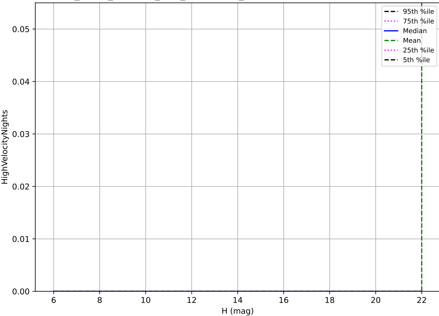
roll_pause_mjdp270_v3.4_10yrs: OCC_r20 High velocity pair detection loss
