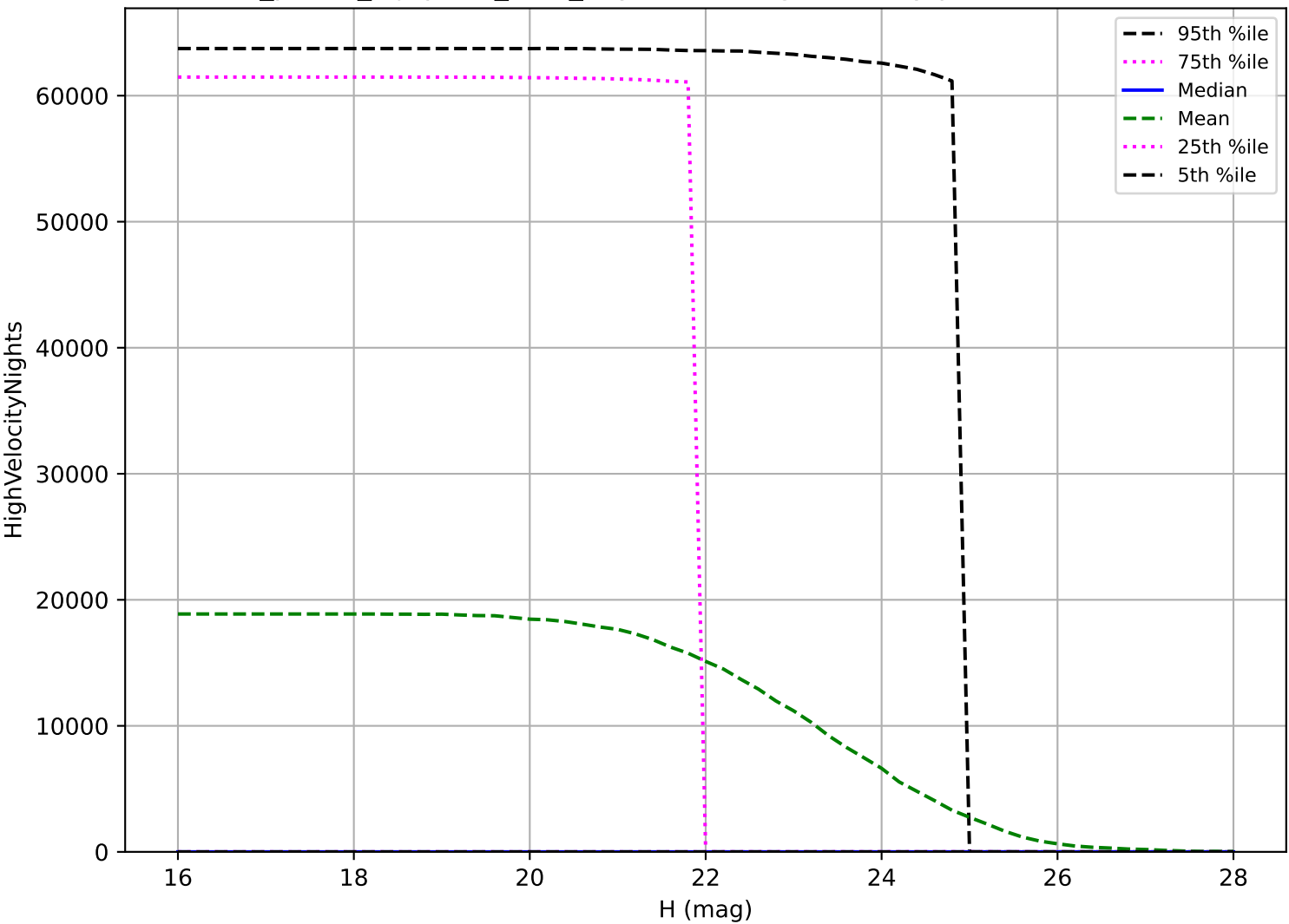
roll_pause_mjdp270_v3.4_10yrs: NEO High velocity pair detection loss
