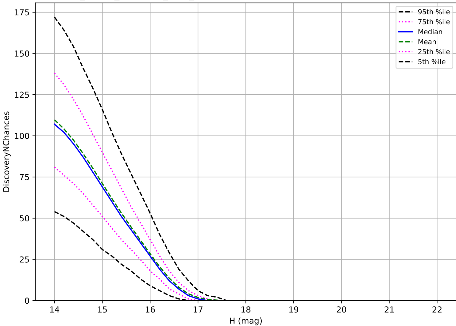
roll_pause_mjdp270_v3.4_10yrs: Trojan 3 pairs in 15 nights detection loss
