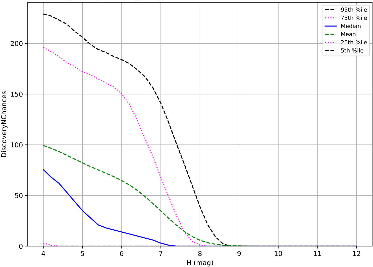
roll_pause_mjdp270_v3.4_10yrs: TNO 3 pairs in 15 nights detection loss
