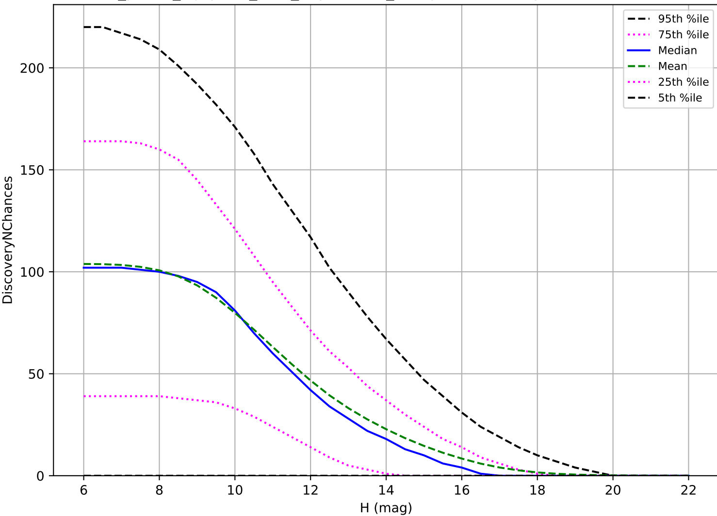
roll_pause_mjdp270_v3.4_10yrs: OCC_r5 3 pairs in 15 nights detection loss
