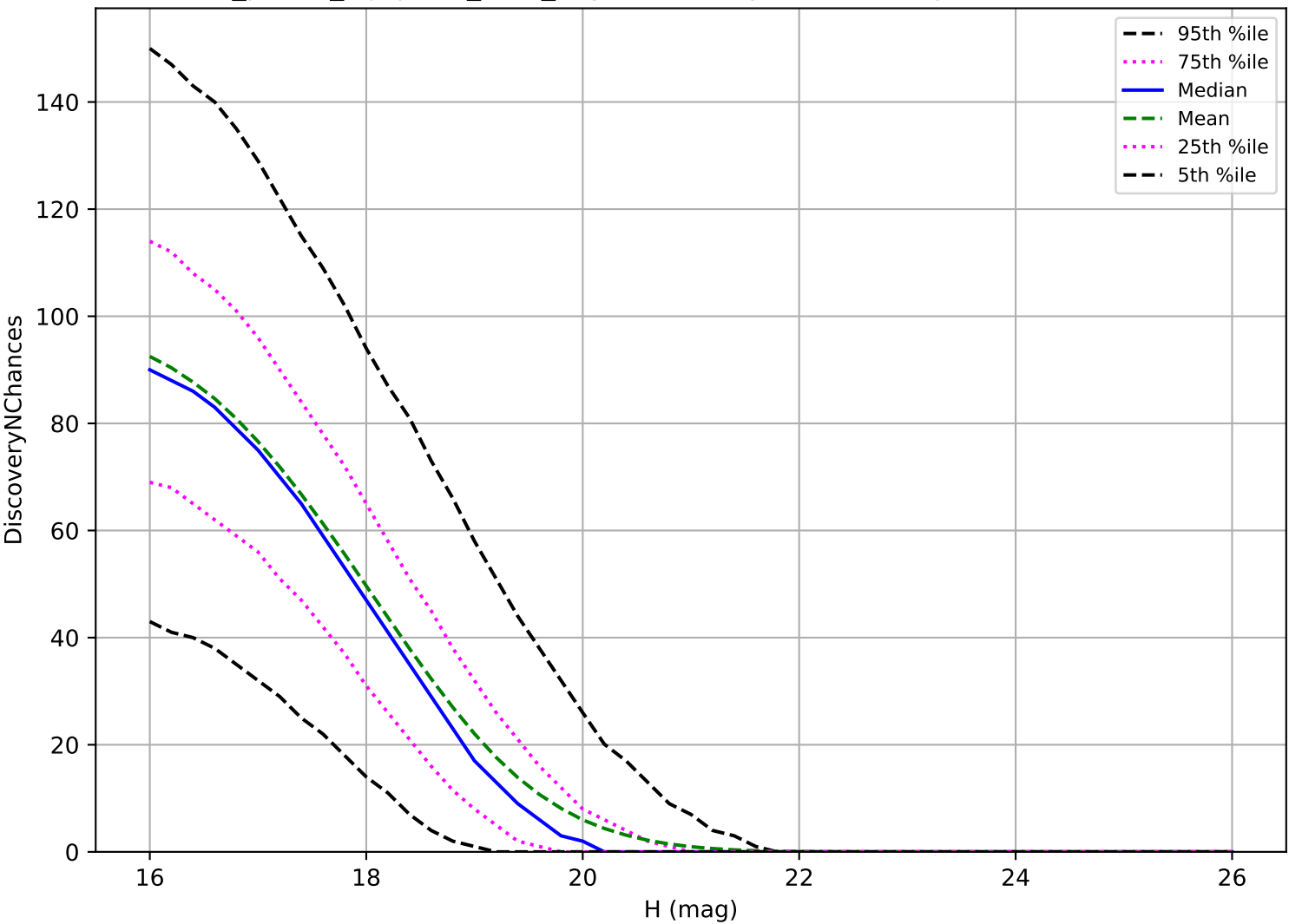
roll_pause_mjdp270_v3.4_10yrs: MBA 3 pairs in 15 nights detection loss
