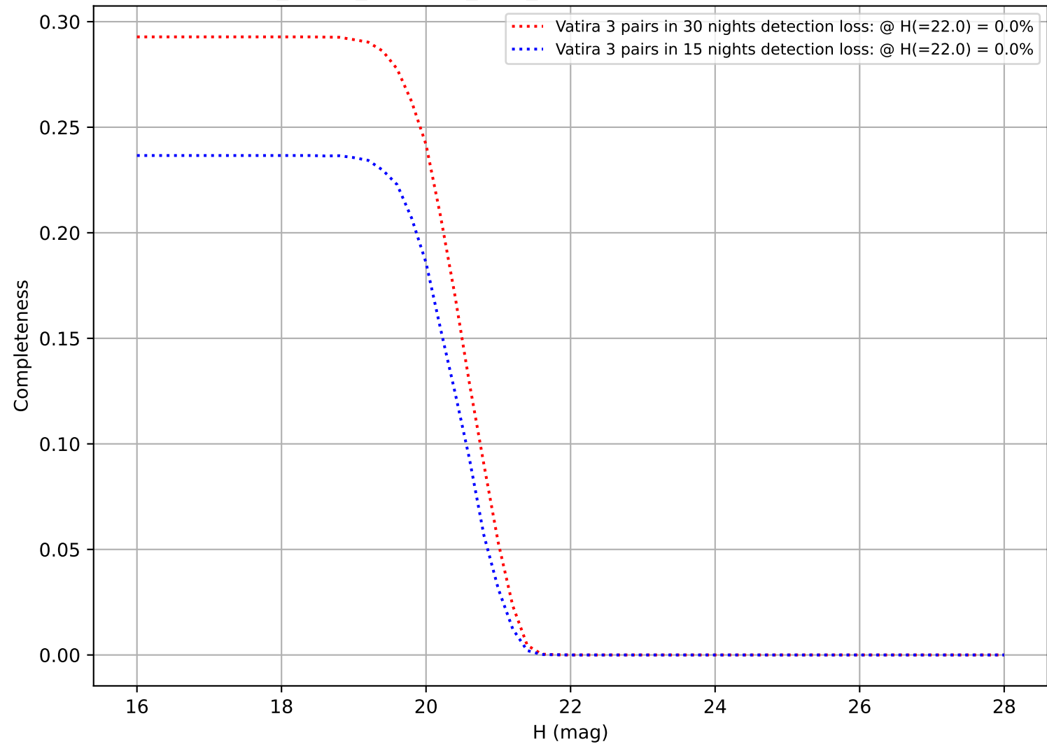
roll_pause_mjdp270_v3.4_10yrs: DifferentialCompleteness
